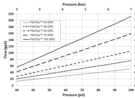
Figure 1: Impact of Pressure on Target Permeate Flow (constant temperature, recovery)
