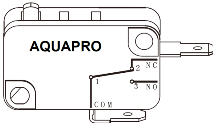
INTERNAL MICRO SWITCH
