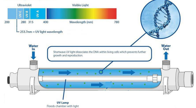
Electromagnetic Spectrum
